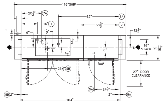
Plan View: Right to Left Model
