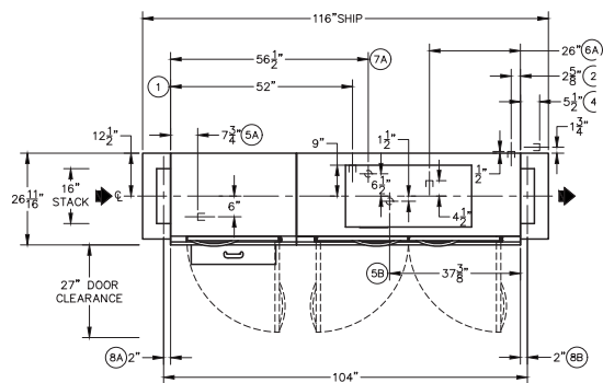
Plan View: Left to Right Model
