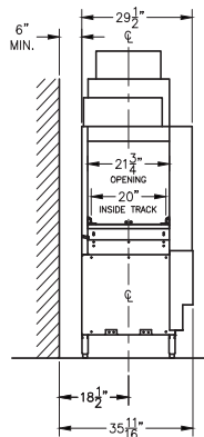
End View
