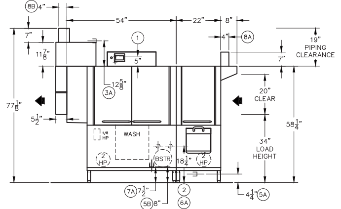
Front View: Right to Left Model R-L
