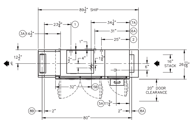
Plan View: Right to Left Model R-L
