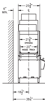
End View
