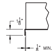
Flange Details
