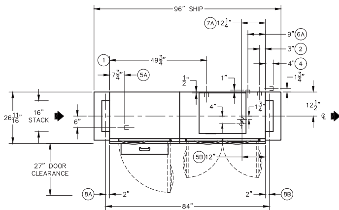
Plan View: Left to Right Model L-R
