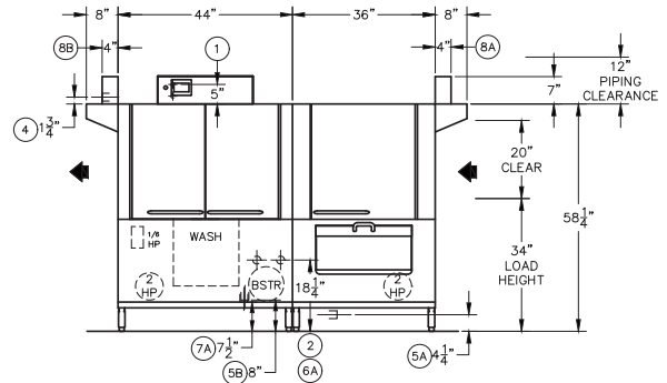
Front View: Right to Left Model R-L
