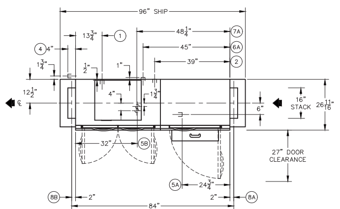
Plan View: Right to Left Model R-L
