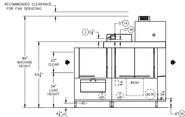
Front View: Left to Right Model
